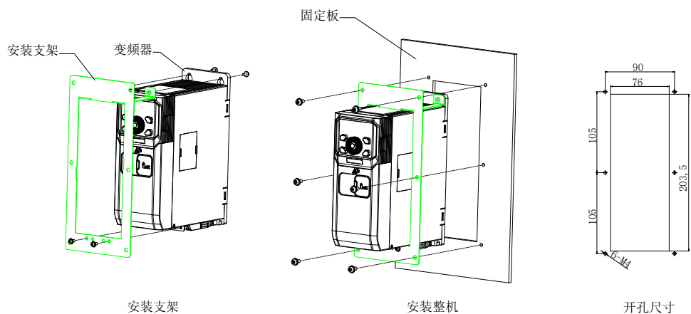
图2-33 MV810-EMBB (适用于0.37~3.7kW)
