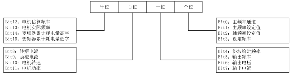
图7-48 LED运行显示参数选择1设定
